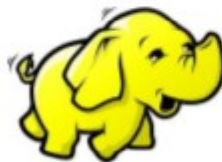
Hadoop
