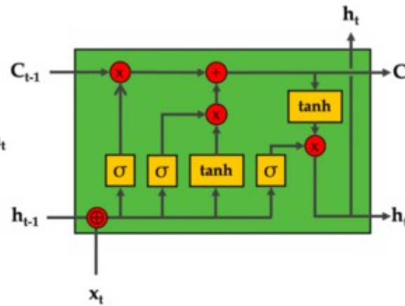
LSTM
