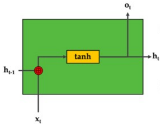
RNN
